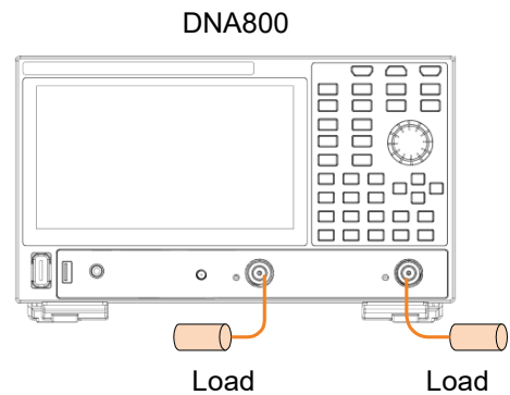
Figure 4.2 Test Device Connection for Effective Directivity
