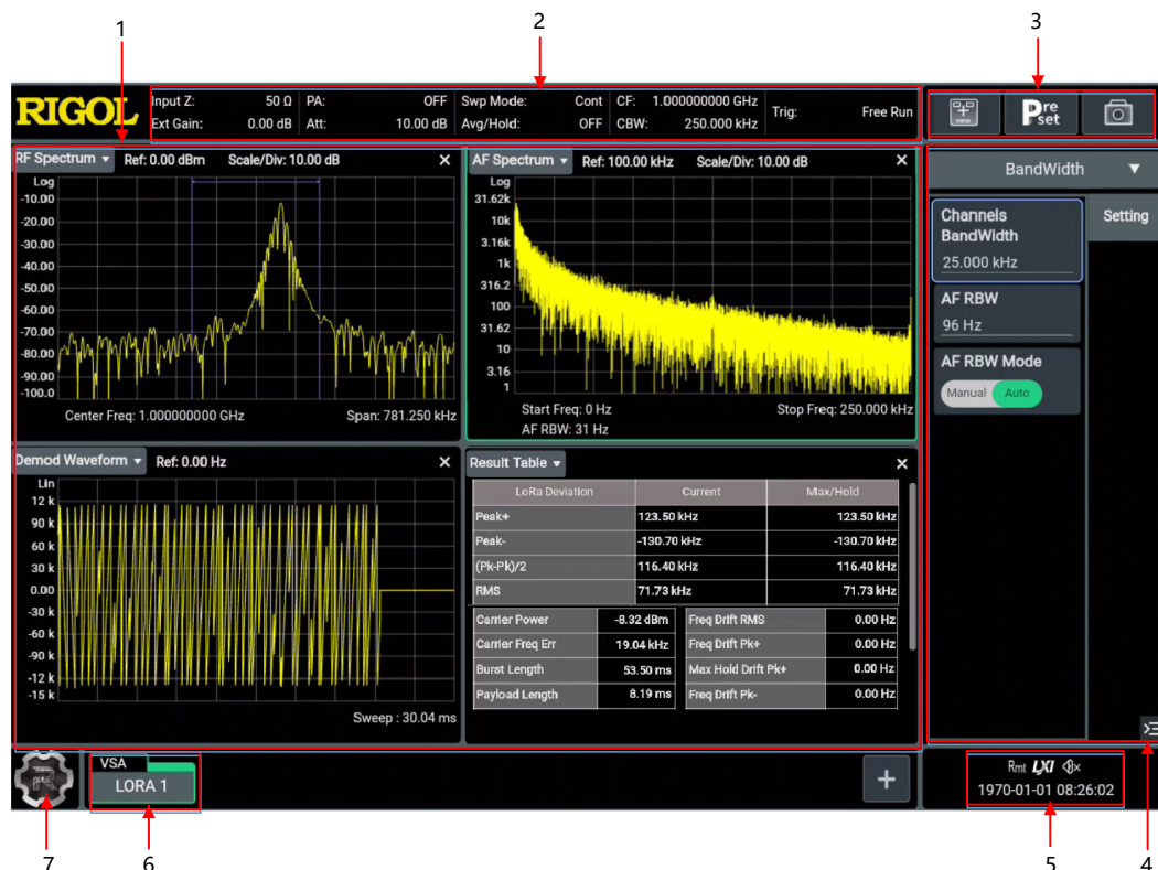
Figure 3.1 User Interface
